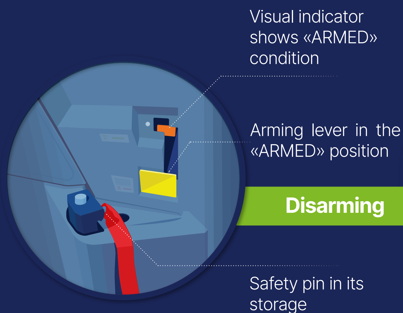
Figure: ARMED/DISARMED conditions for A320 Family cabin door
